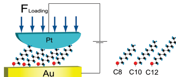
Scheme 1. Schematic of a Molecular Junction Using the CAFM Method a
